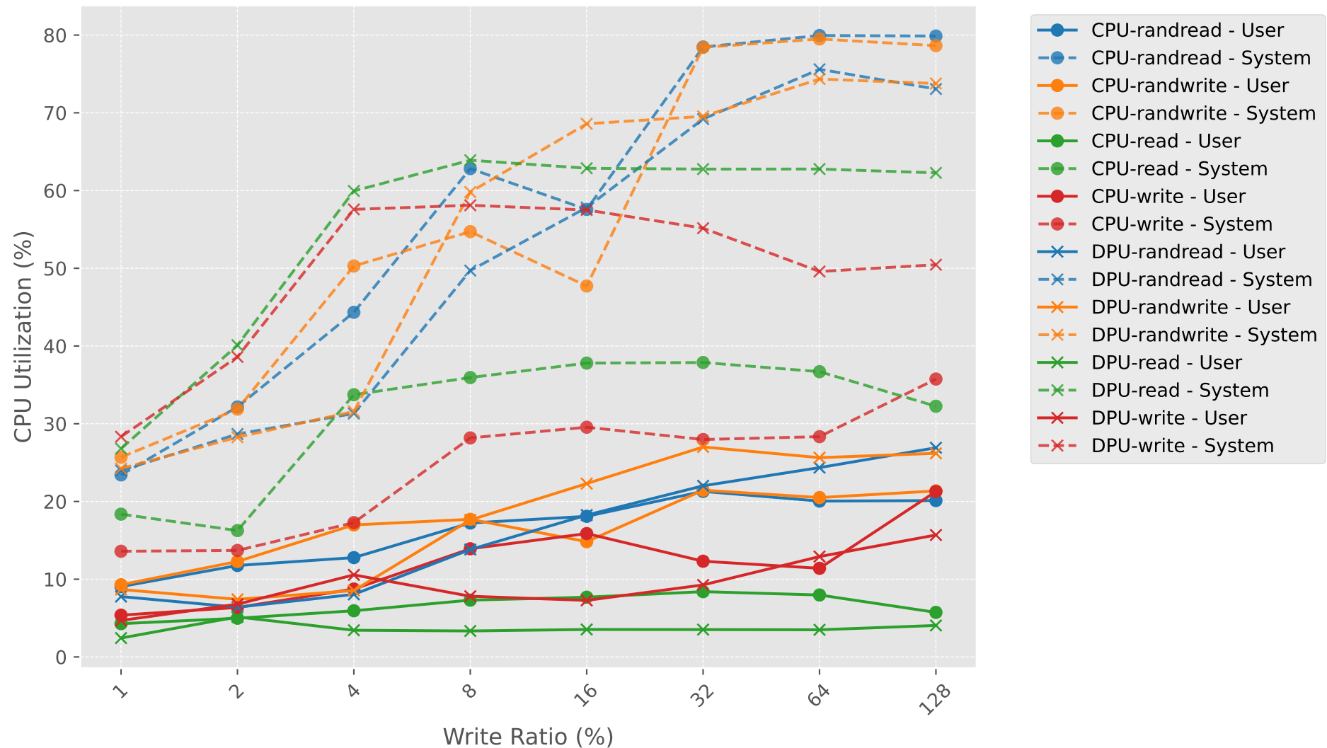
CPU Utilization vs Write Ratio (iodepth)
